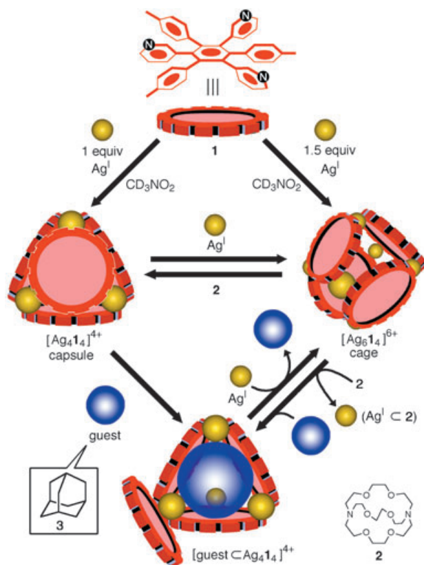
Figure 1. Schematic representation of the interconversion between [Ag 4 L 4 ] 4+ capsule and [Ag 6 L 4 ] 6+ cage complexes by changing the [Ag I ]/[ 1 ] ratio from 1:1 to 1.5:1. The [Ag 4 L 4 ] 4+ capsule complex can entrap a neutral organic molecule such as adamantane in the inner space, while the [Ag 6 L 4 ] 6+ cage complex cannot practically encapsulate the guest molecule. The encapsulation/release of the guest molecule is coupled with the reversible Ag I -dependent capsule↔cage interconversion. A front disk is opened to show clearly a guest molecule encapsulated in the inner space of [guest@Ag 4 L 4 ] 4+ .
