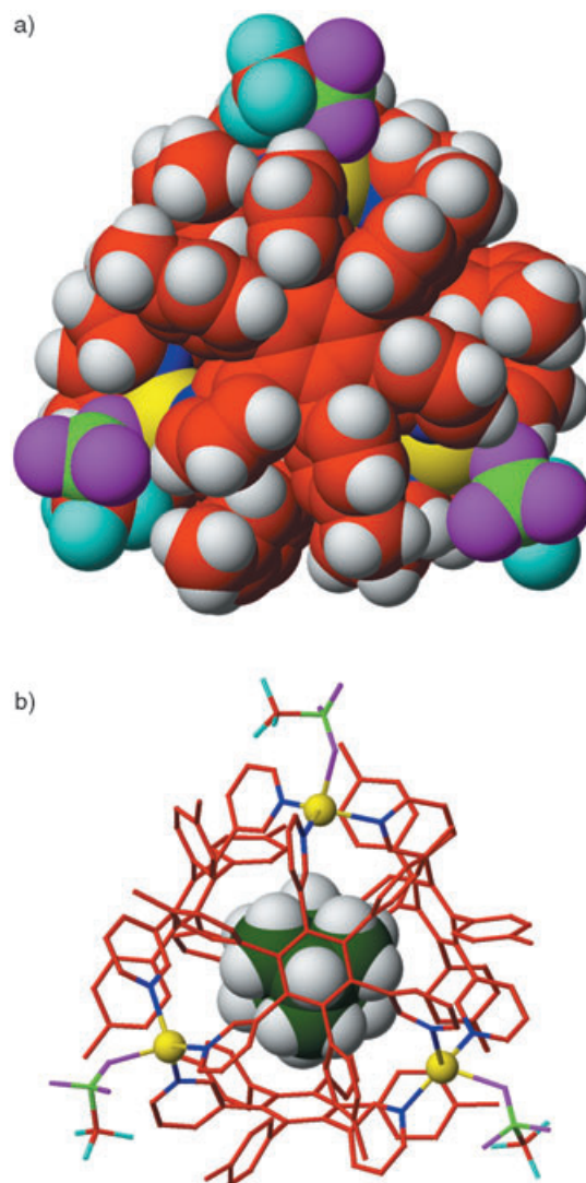
Figure 4. The crystal structure of \text{3CAg}_4\text{L}_4(\text{TfO})_4 . Color labels: red (carbon), turquoise (carbon of 3 ), blue (nitrogen), yellow (silver), purple (oxygen), light green (sulfur), cyan (fluorine), and white (hydrogen). a) A space-filling model; b) the capsule structure is depicted as a cylinder model. Hydrogen atoms of the [\text{Ag}_4\text{L}_4]^{4+} moiety are omitted for clarity.
