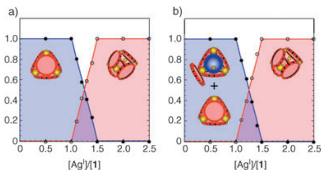
Figure 3. Effects of the presence of adamantane ( 3 ) on the inter-conversion between [\text{Ag}_4\text{L}_4]^{4+} and [\text{Ag}_6\text{L}_4]^{6+} . a) Plot of [\text{Ag}_4\text{L}_4]/([\text{Ag}_4\text{L}_4] + [\text{Ag}_6\text{L}_4]) (filled circles) and [\text{Ag}_6\text{L}_4]/([\text{Ag}_4\text{L}_4] + [\text{Ag}_6\text{L}_4]) (open circles) against [\text{Ag}^+]/[\text{L}] determined from the ^1\text{H} NMR integral ratios. Solid lines are theoretically drawn for [\text{Ag}_4\text{L}_4]/([\text{Ag}_4\text{L}_4] + [\text{Ag}_6\text{L}_4]) (blue) and [\text{Ag}_6\text{L}_4]/([\text{Ag}_4\text{L}_4] + [\text{Ag}_6\text{L}_4]) (red) as a function of [\text{Ag}^+]/[\text{L}] . b) Plot of ([\text{3CAg}_4\text{L}_4] + [\text{Ag}_4\text{L}_4])/([\text{3CAg}_4\text{L}_4] + [\text{Ag}_4\text{L}_4] + [\text{Ag}_6\text{L}_4]) (filled circles) and [\text{Ag}_6\text{L}_4]/([\text{3CAg}_4\text{L}_4] + [\text{Ag}_4\text{L}_4] + [\text{Ag}_6\text{L}_4]) (open circles) against [\text{Ag}^+]/[\text{L}] determined from the ^1\text{H} NMR integral ratios. Solid lines are theoretically drawn as a function of [\text{Ag}^+]/[\text{L}] . A front disk is opened to clearly show a guest molecule in the inner space for the [\text{3CAg}_4\text{L}_4]^{4+} complex.
