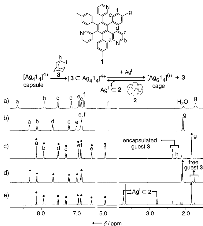
Figure 2. a)–b) ^1\text{H} NMR spectra (500 MHz) of [\text{Ag}_4\text{L}_4]^{4+} capsule and [\text{Ag}_6\text{L}_4]^{6+} cage complexes ( \text{CD}_3\text{NO}_2 , 293 K, [\text{I}] = 5.9 \text{ mM} ); a) \text{Ag}_4\text{L}_4(\text{PF}_6)_4 and b) \text{Ag}_6\text{L}_4(\text{PF}_6)_6 . c)–e) Encapsulation of a guest molecule 3 in the [\text{Ag}_4\text{L}_4]^{4+} capsule complex and encapsulation/release of the guest molecule triggered by the capsule \leftrightarrow cage interconversion ( ^1\text{H} NMR ( \text{CD}_3\text{NO}_2 , 273 K, [\text{I}] = 10.8 \text{ mM} ); c) [\text{3C Ag}_4\text{L}_4]^{4+} , [\text{Ag}_4\text{L}_4(\text{PF}_6)_4] = [\text{3}] = 2.7 \text{ mM} . d) Upon addition of \text{AgPF}_6 (2.0 equiv) to the sample for (c), encapsulated 3 was released from inside as a result of the interconversion from the capsule into the cage. e) Upon addition of [2,2,2]cryptand 2 (2.0 equiv) to the sample for d), an \text{Ag}_4\text{L}_4 capsule complex was formed and 3 was immediately encapsulated again in the capsule. Filled circles and triangles denote the inclusion complex [\text{3C Ag}_4\text{L}_4]^{4+} and the [\text{Ag}_6\text{L}_4]^{6+} cage complex, respectively.
